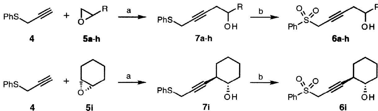
Scheme 1. Synthesis of compounds 6a-i from phenyl propargylic sulfide 4 and epoxides 5a-i .
