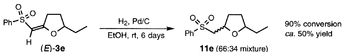
Scheme 3. Catalytic hydrogenation of 3e .
