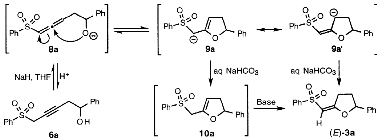
Scheme 2. Base-induced cyclization of hydroxyl propargylic sulfone 6a .
